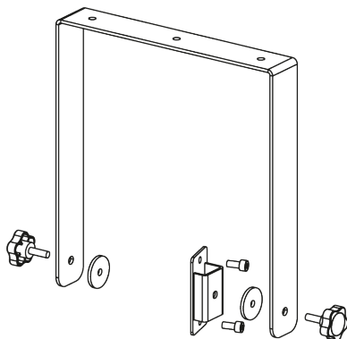
LDEB122G2SB / LDEB152G2SB Swing Bracket
